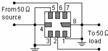
Test Circuit
