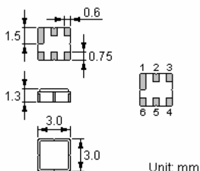
Ceramic Package: DCC6C
