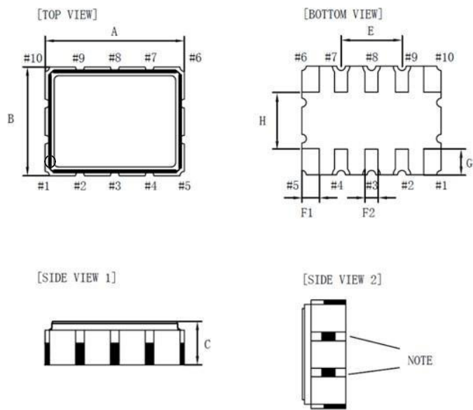
Figure 1. Dimensions
