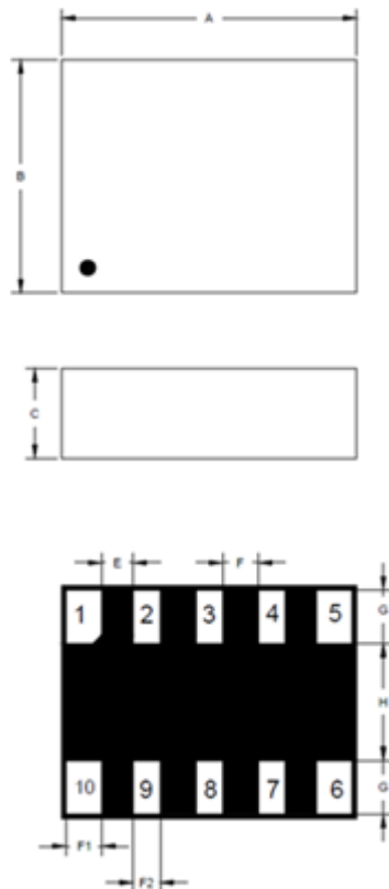
Figure 5. Dimension
