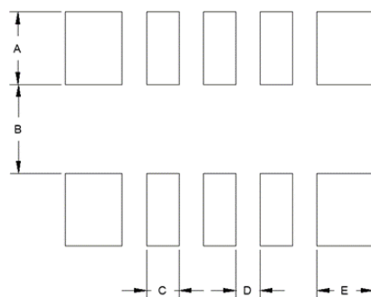
Figure 6. Recommended Soldering Pattern
