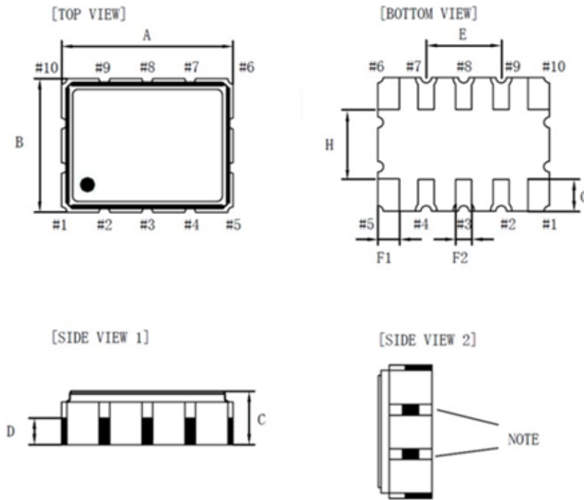
Figure 3. Dimensions
