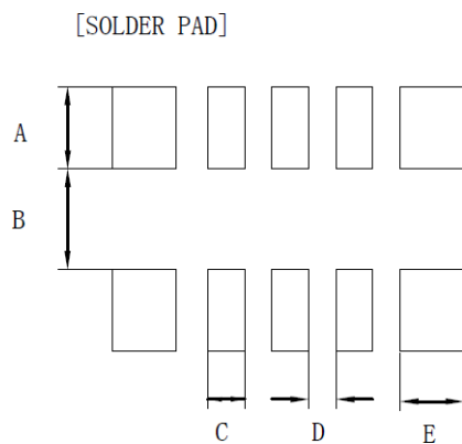
Figure 4. Recommended Solder Pad
