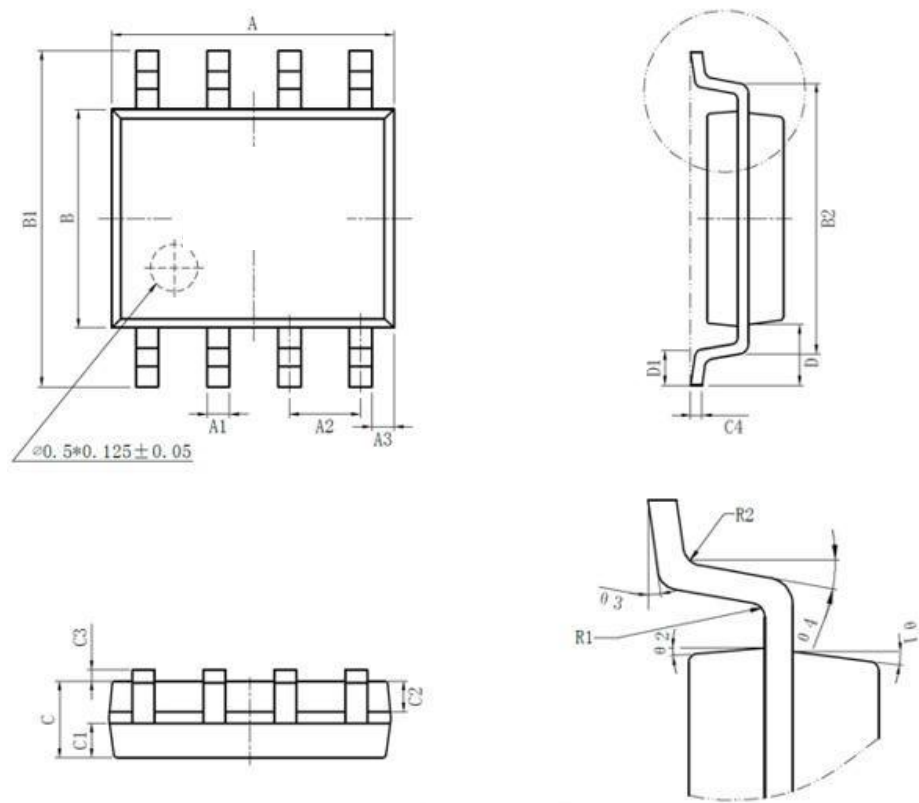
Figure 4. Dimension
