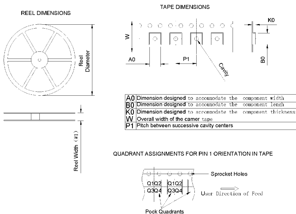
Figure 5. Package information
