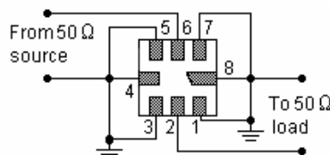
Test Circuit
