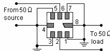
Test Circuit
