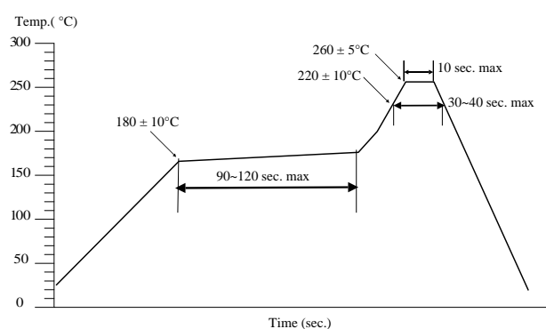
Reflow profile
