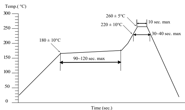
Reflow profile
