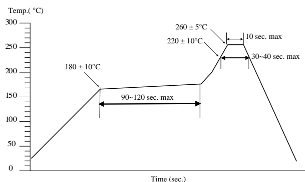
Reflow profile
