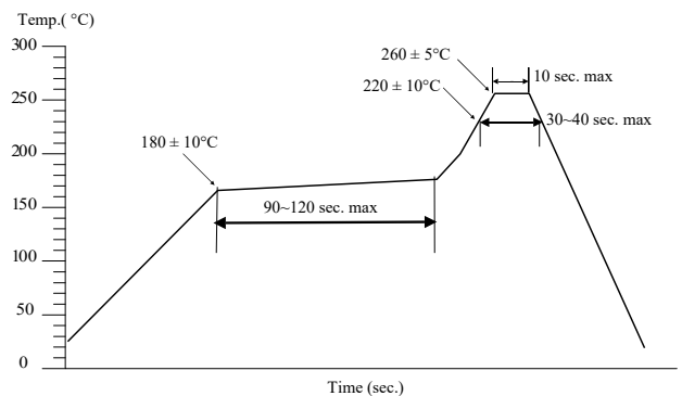
Reflow profile
