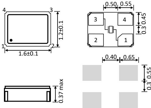
Dimensions (mm)
